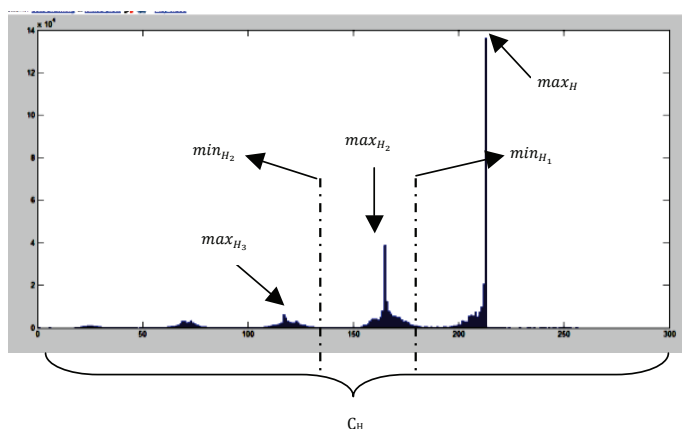
Figure 1. The image histogram of the Intensity of Image Histogram (IIH-Met) shows the three highest peaks in the image, namely \max_H , and C_H is the intensity's pixel values on image histogram, which is the highest peak; \max_{H2} , the second highest; and \max_{H3} , the third highest peak in the image and C_H is the intensity's pixel values on image histogram
